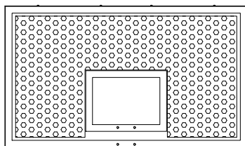
SR-PERF / AL-PERF ALUMINUM OR STEEL PERFORATED BOARD REAR BRACING INCLUDED
