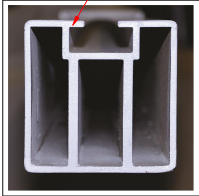
4" x 4" EXTRUDED HEAVY WALL ALUMINUM WITH ADDITIONAL LATERAL SUPPORT
