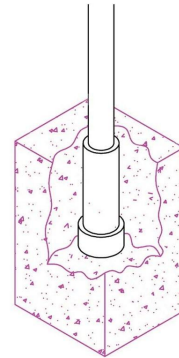
INCLUDES 18" DEEP GROUND SLEEVE*
